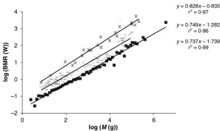
Fig. 2. Plots of the basal (Hart 1971; Heusner 1991; Lovegrove 2000; Lovegrove 2003; White & Seymour 2003), field (Nagy et al. 1999) and maximal metabolic rates (Pasquis et al. 1970; Hart 1971; Lechner 1978; Prothero 1979; Taylor et al. 1981; Taylor et al. 1988; Bishop 1999; Sapoval et al. 2002). The regression lines are fitted to the average of the logarithms for every 0.1 log unit interval of mass. This was done in order to give equal weighting to big and small mammals. For the basal metabolic rate only the averages are shown because the raw data is shown in Fig. 1. Both raw and averaged data for basal metabolic rate are shown in Fig. 1, but here only the averages (filled squares) are shown. For the field and maximal data, diamonds and stars are the average data, and bars and open squares are the raw data, respectively. While the slope for the maximal metabolic rate is slightly higher than that for the field or basal rates, all of the slopes are close to 3/4 . The slope for basal is b = 0.737 ( P < 0.0001 , n = 52 , 95% CI 0.711, 0.762), for field is 0.749 ( P < 0.0001 , n = 35 , 95% CI 0.697, 0.801), and for maximal is 0.828 ( P < 0.0001 , n = 21 , 95% CI 0.758, 0.897).
