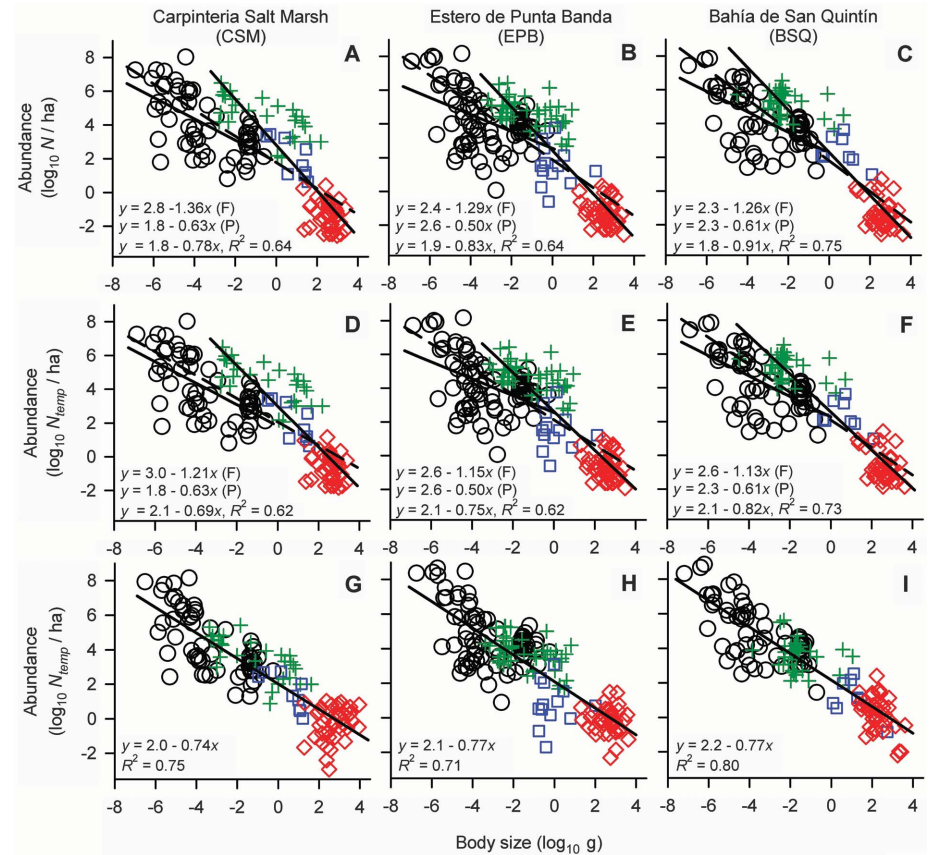
Fig. 1. Abundance as a function of body size for parasitic and free-living species in three estuaries: Carpinteria Salt Marsh (CSM), Estero de Punta Banda (EPB), and Bahía de San Quintin (BSQ). (A to C) Abundance versus body size reveals that a single regression line cannot adequately fit the data (general linear models: all interaction P s < 0.0001; tables S2 and S3). Solid lines and top two equations give the slopes and intercepts for parasitic (P) and free-living (F) species; slope 95% confidence limits: CSM, \pm 0.14 ; EPB, \pm 0.13 ; BSQ, \pm 0.11 . The broken lines, bottom equations, and R^2 s pertain to pooled data. (D to F) Temperature-corrected abundance versus body size gives relationships very similar to those seen in (A) to (C), although bird abundance is shifted up by about half an order of magnitude, leading to slightly shallower slopes for free-living and pooled data. Lines and equations as in (A) to (C); slope 95% confidence limits: CSM, \pm 0.13 ; EPB, \pm 0.12 ; BSQ, \pm 0.10 . (G to I) Temperature-corrected abundance versus body size, statistically controlling for trophic level (Fig. 3 and tables S4 and S5). The scaling slopes are all consistent with the -3/4 predicted by metabolic scaling, as slightly modified for the distribution of the number of species along the body-size axis (11); slope 95% confidence limits: CSM, \pm 0.073 ; EPB, \pm 0.073 ; BSQ, \pm 0.063 . The R^2 values represent partial R^2 s for body size. Symbol key for all figures: circles, parasites; crosses, invertebrates; squares, fish; diamonds, birds.
