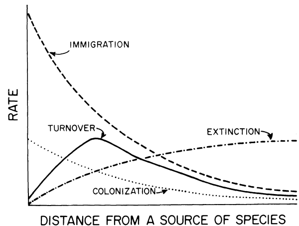
FIG. 2. A graphical representation of the relationship between the distance to a source of species and turnover rate at equilibrium. Note that rates of immigration and colonization decrease with insular isolation as suggested by MacArthur and Wilson; but, in contrast to their model, extinction rate increases with isolation because of the rescue effect. The result is that equilibrium turnover rate first increases and then decreases with distance from a source of species, and turnover is greatest where both colonization and extinction rates are high. The shapes of these curves are hypothetical and should vary with the characteristics of particular insular systems.
