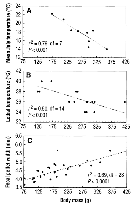
Fig. 1. Scatterplots and linear regression equations showing variation in characteristics of woodrats as a function of body mass. (A) Relation between adult body mass and average July temperature in nine contemporary populations of N. cinerea from western Northern America. Data are taken from museum specimens and from unpublished field notes. Values represent location means of a minimum of 20 individuals. Weather data were taken from the U.S. Historical Climatology Network and generally represent a minimum of a 50-year average. We used a terrestrial lapse rate of -0.5^{\circ}\text{C} per 100 m to correct for elevational differences between collection sites of locations in Northern California and the nearest weather station. Only a weak relation was observed between body mass and average January temperatures (23). (B) Relation between body mass and upper lethal temperature for 16 individual N. cinerea representing several populations; data were taken from (24). (C) Relation between body mass and the average width of fecal pellets for three woodrat species: N. cinerea , N. lepida , and N. albigula . A total of 30 field-trapped animals (10 per species) were housed in the laboratory under a constant temperature and light regime ( 20^{\circ}\text{C} ; 12 hours light, 12 hours dark) and fed a diet of 40% fiber. Fecal pellets were collected, dried, and later measured in a blind study. A linear model provides the best fit ( y = 0.005x + 3.559 ; r^2 = 0.69 ; P < 0.0001 ; partial F test). The size of a fecal pellet can be used to estimate adult body mass with a prediction error of only 21%; diet does not appreciably alter the relation (13). Little of the variation is attributable to species or gender (analysis of covariance, P \gg 0.05 ).
